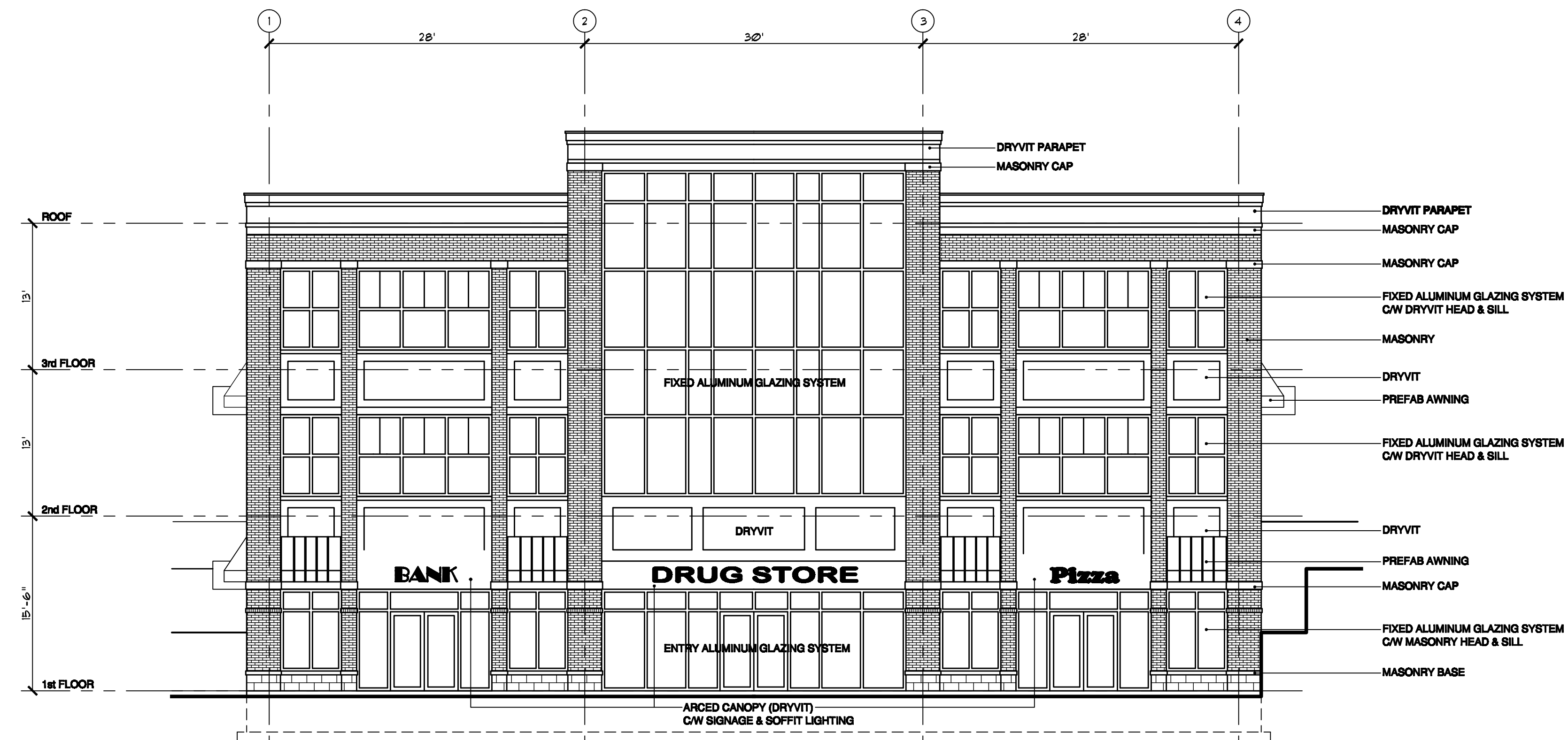
BLDG. A REAR ELEVATION (LOWER PARKING LOT)
